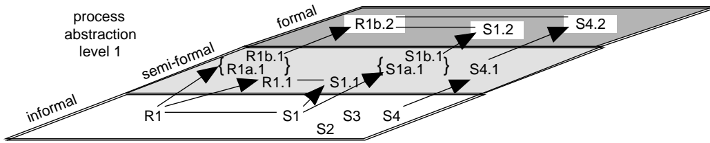
Fig. 4. Traceability relationships depicting the situation when R1b.2 is determined to be incorrect.
