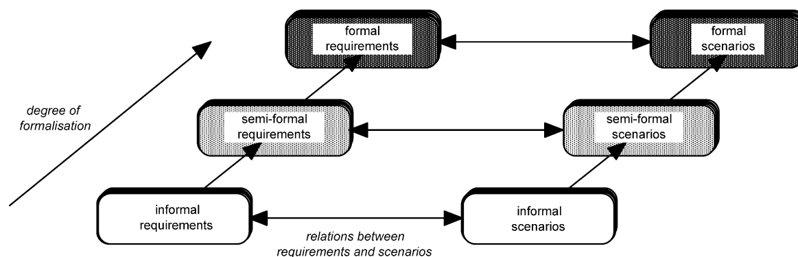
Fig. 1. Representations from informal to formal.
