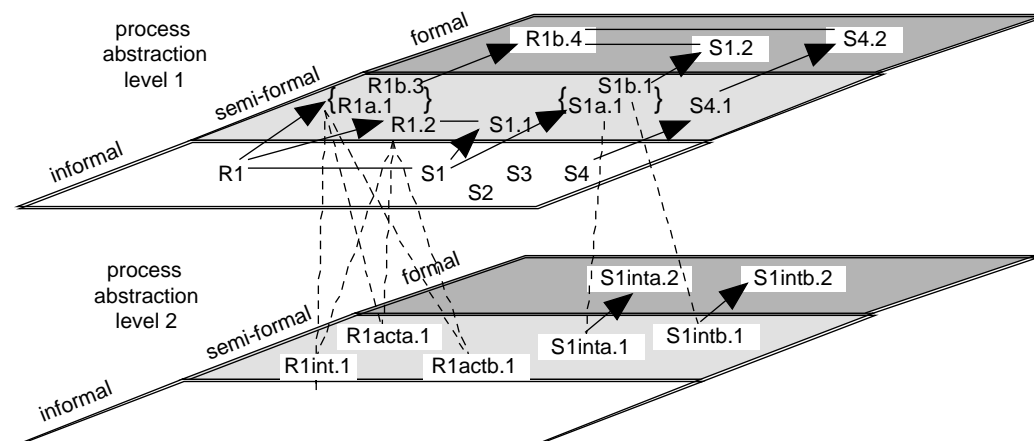
Fig. 6. Traceability relationships for two levels of process abstraction.
