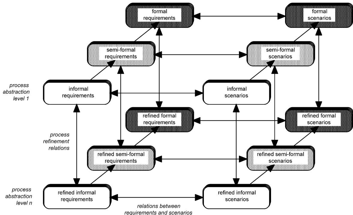
Fig. 3. Traceability relations.
