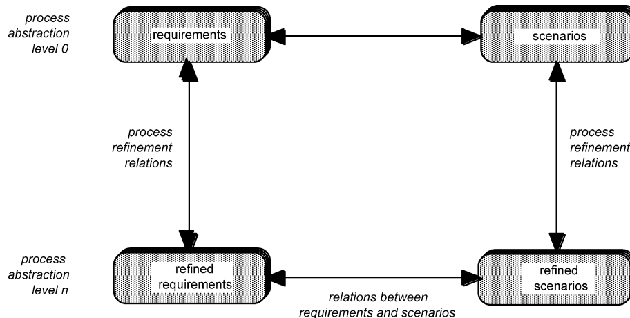
Fig. 2. Process abstraction level refinements
