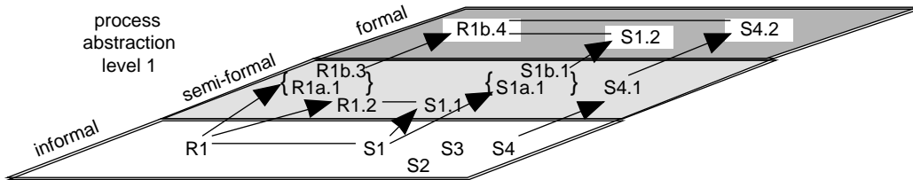
Fig. 5. Traceability relationships depicting the correct requirements and scenarios.
